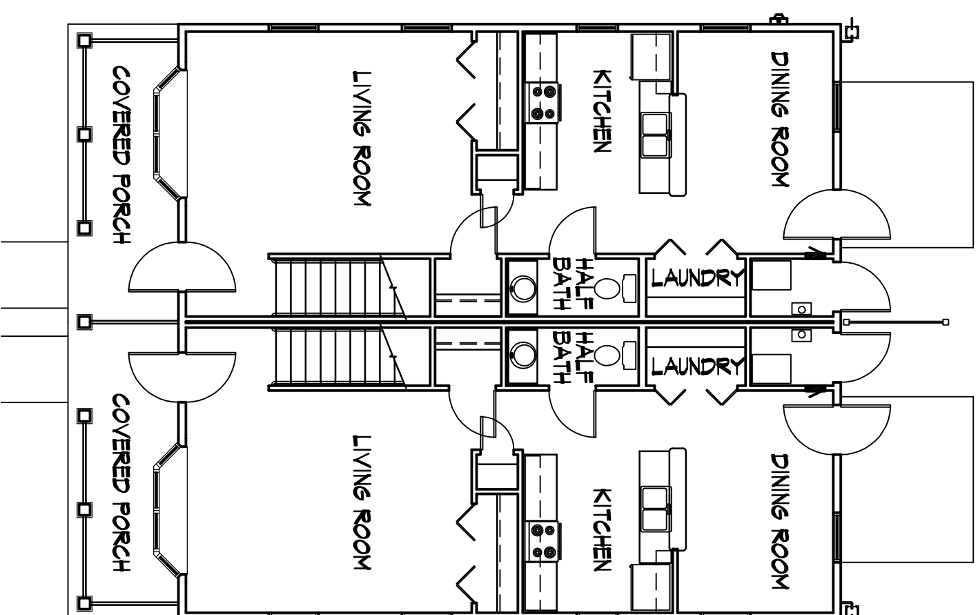
BUILDING "F" MAIN FLOOR 672 SQ. FT. PER UNIT
